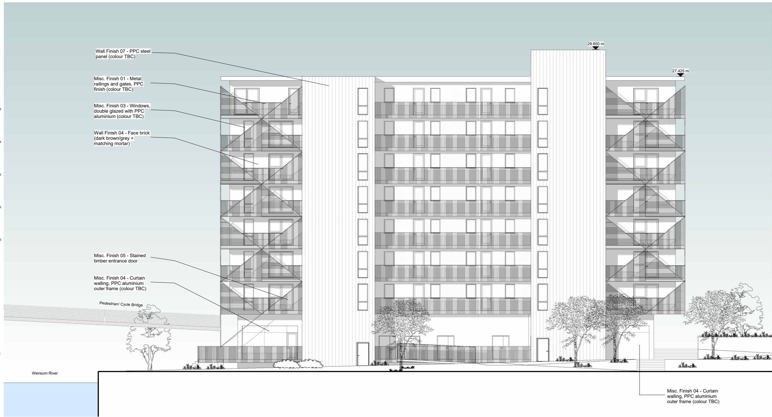
1 West Elevation 1 : 100
