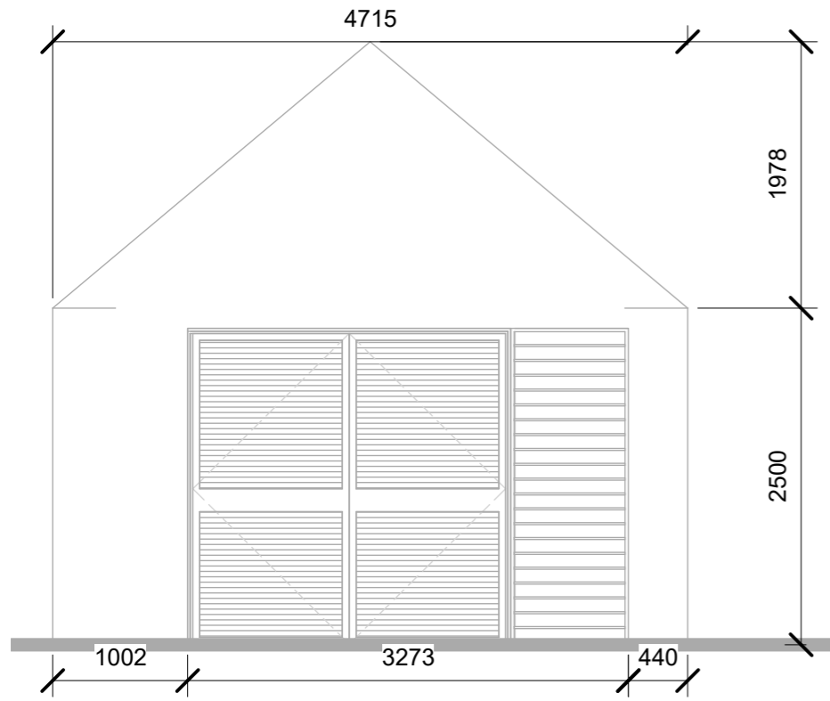
5 Front Elevation 1:50
