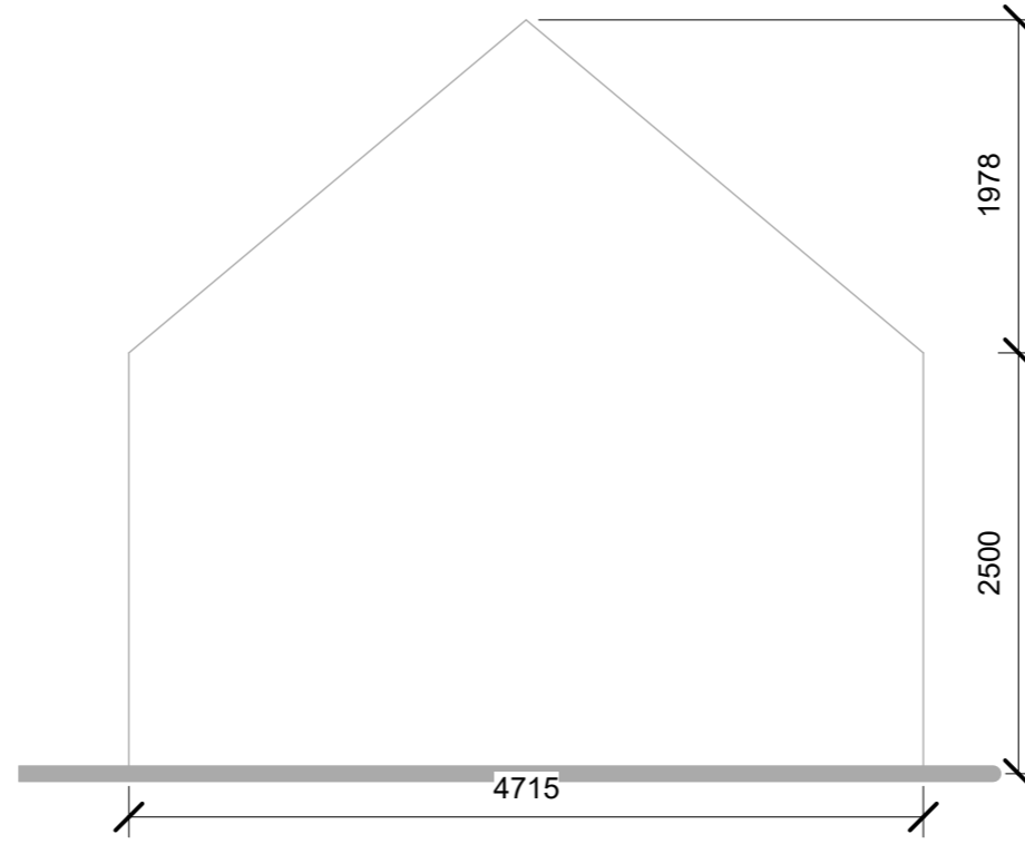
3 Back Elevation 1:50
