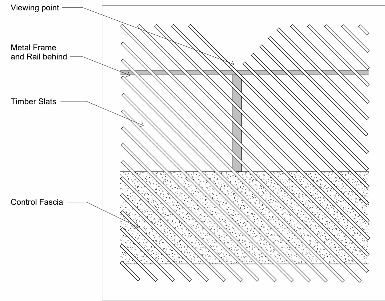
1:25 Bridge Elevation Detail
