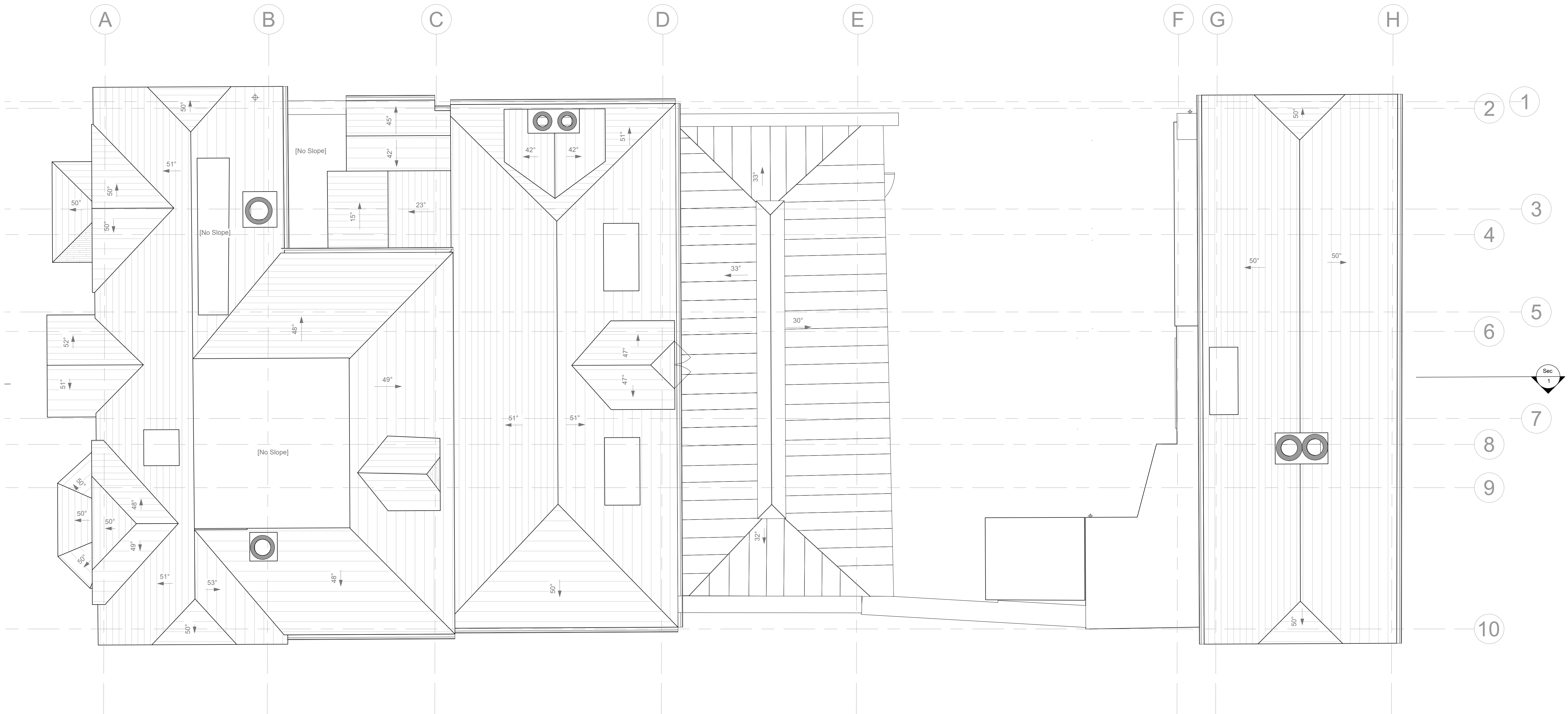
1 Roof Plan 1054 1:50 0 1 2.5 Scale 1:50 m
