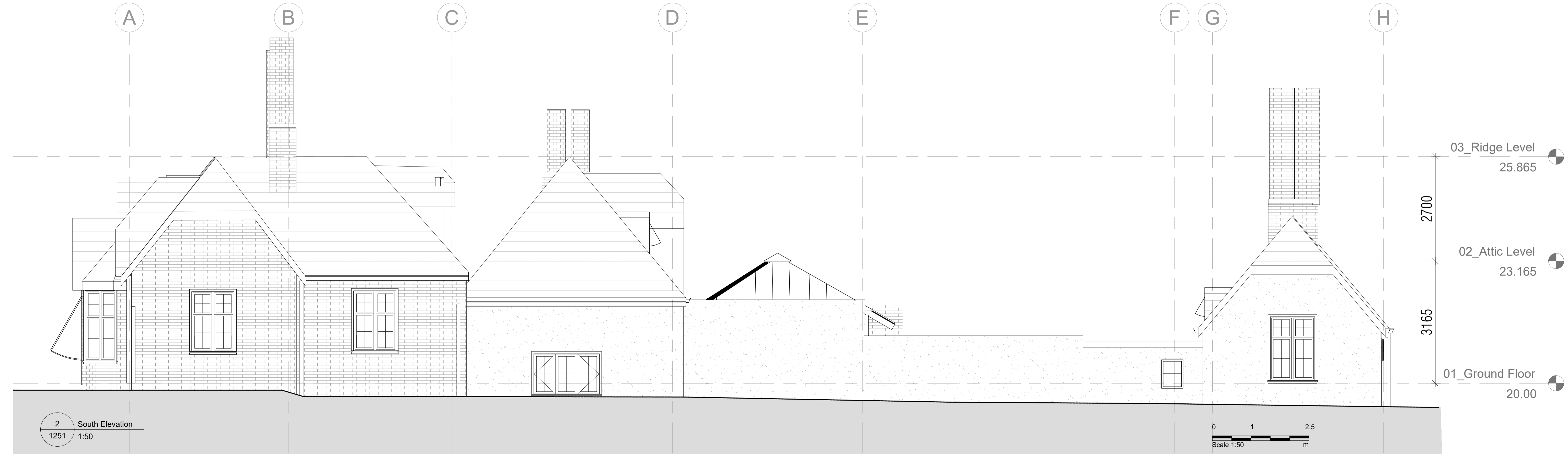
1 North Elevation 1251 1:50
