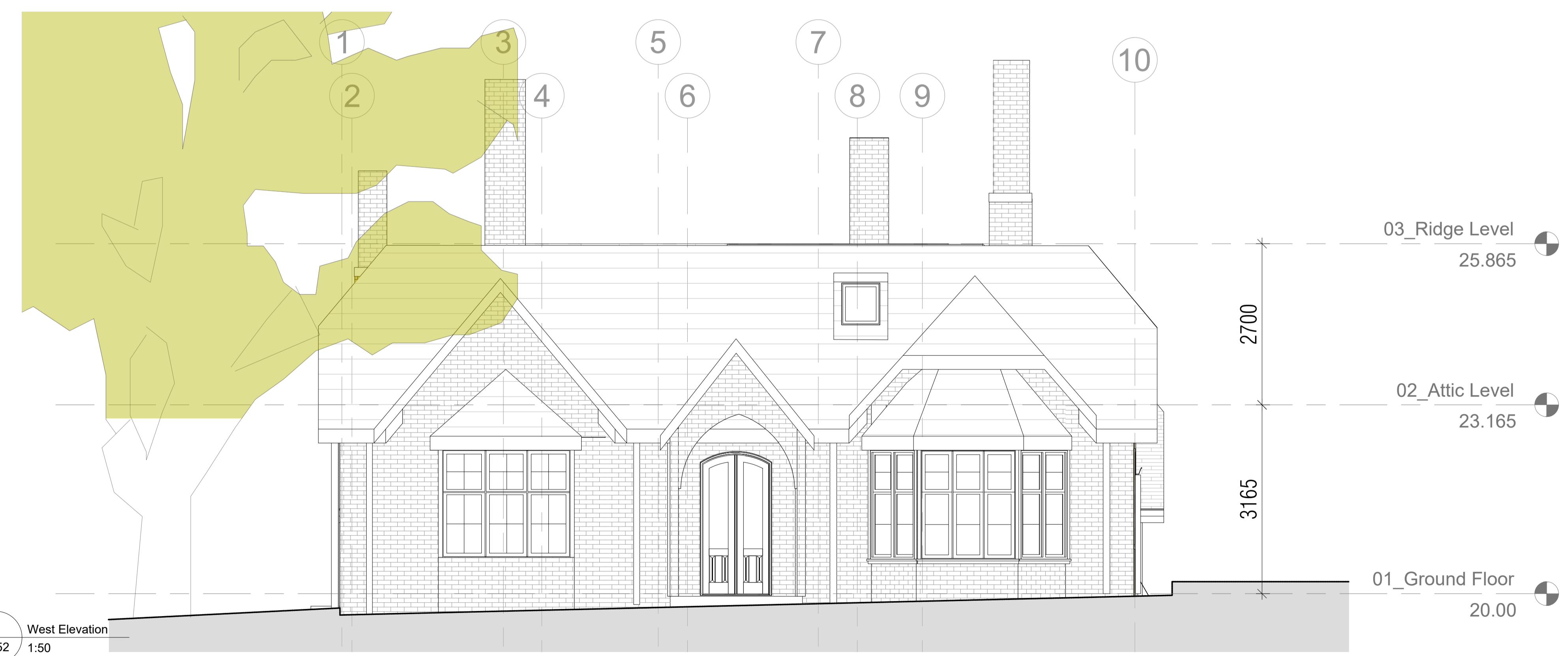
1 East Elevation 1252 1:50
