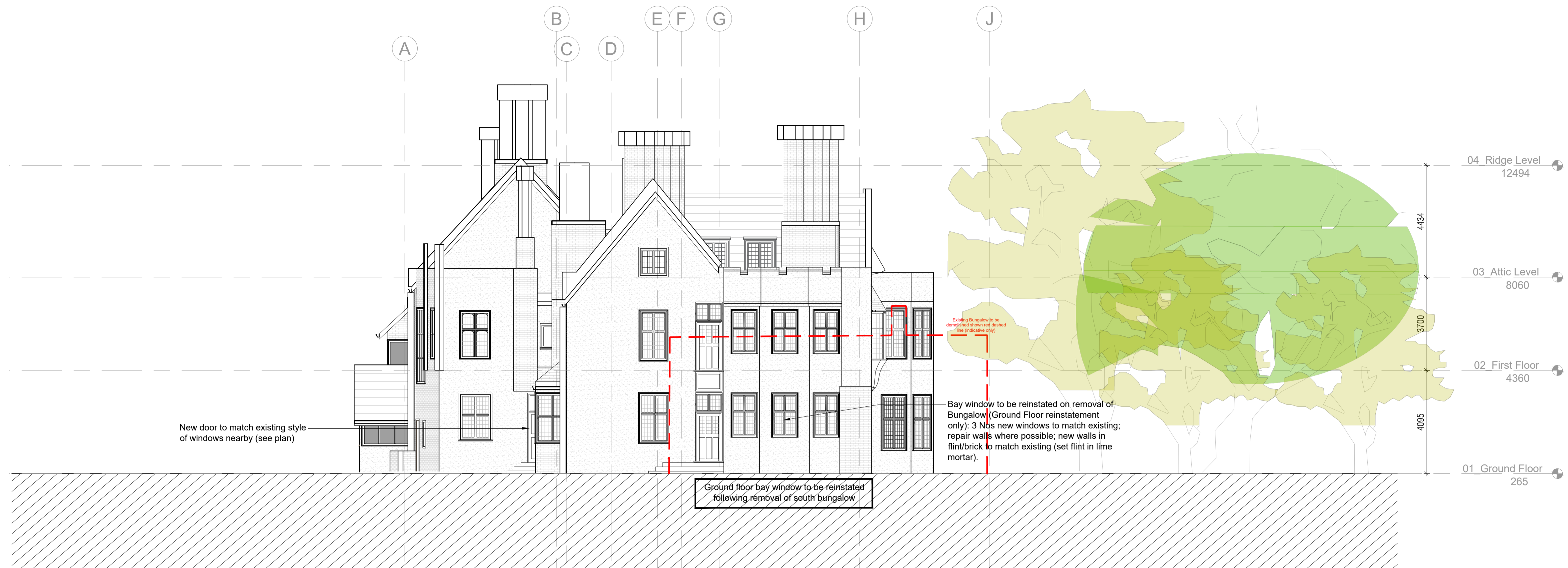
1 South Elevation (To Car Park) 2201 1:100
