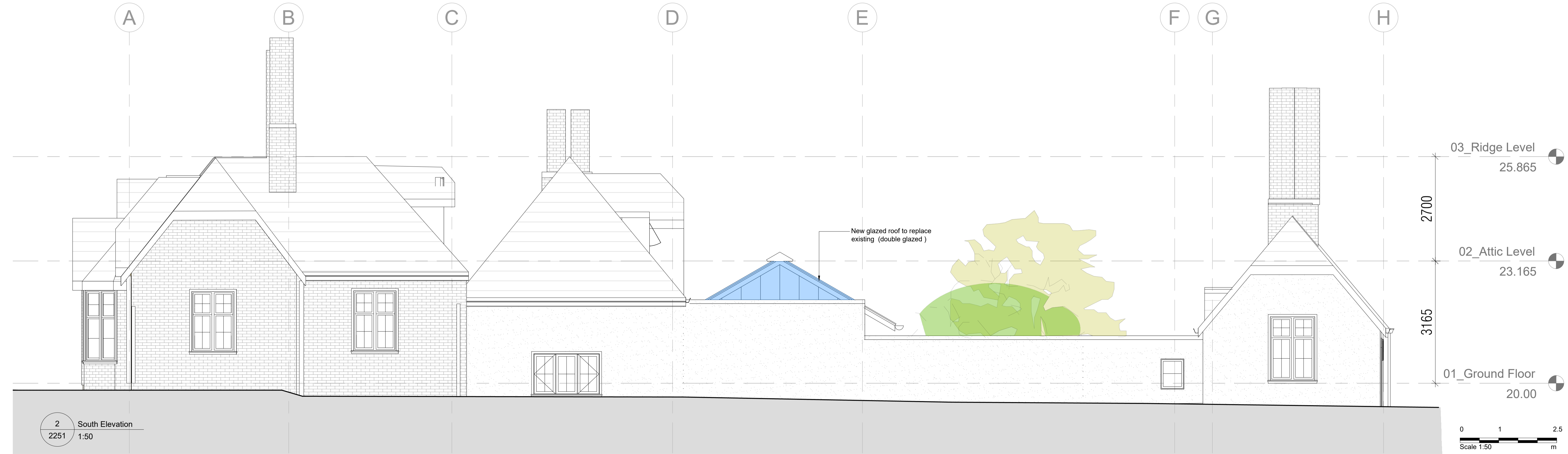
1 North Elevation 2251 1:50
