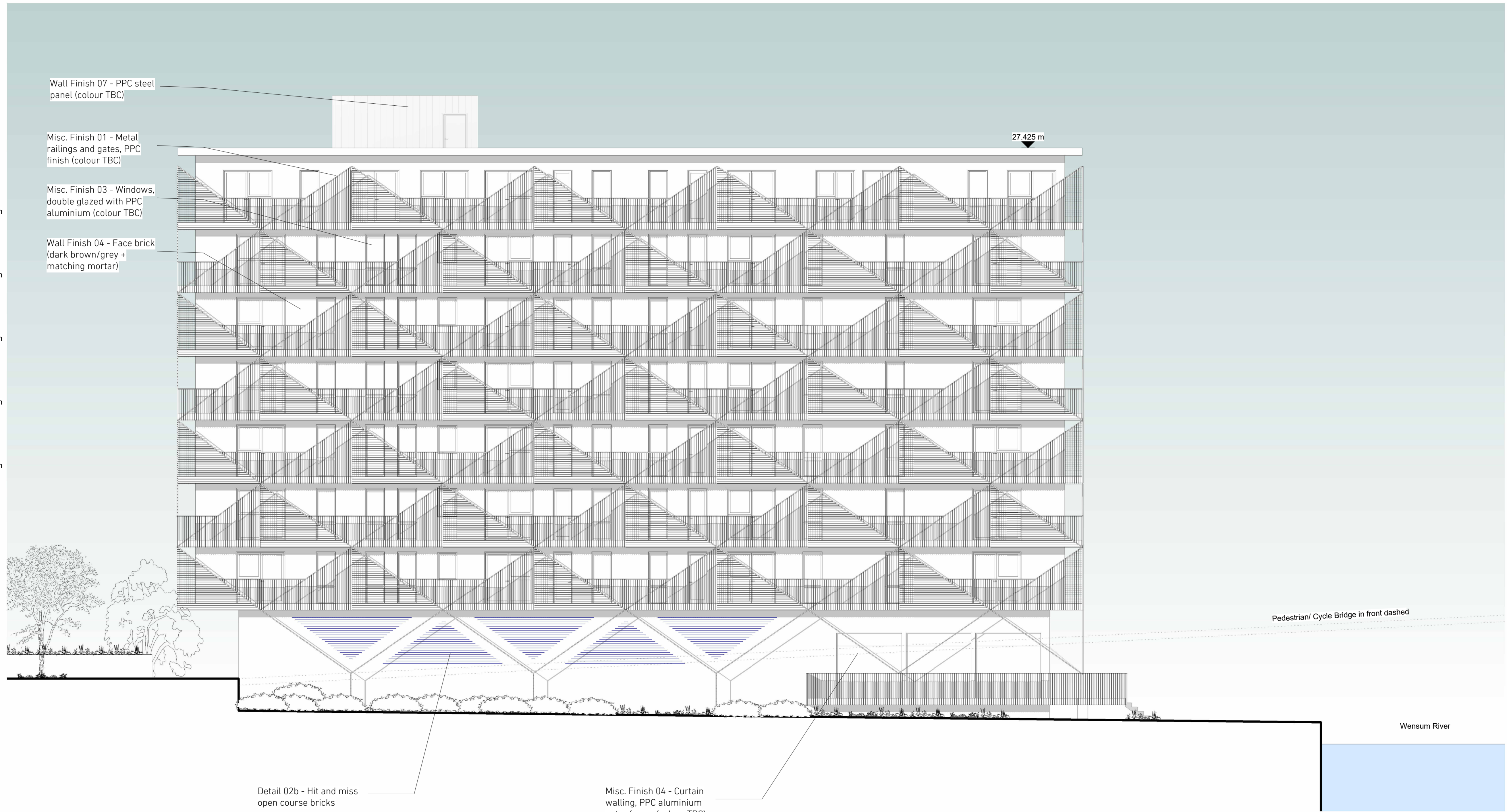
1 East Elevation 1 : 100
